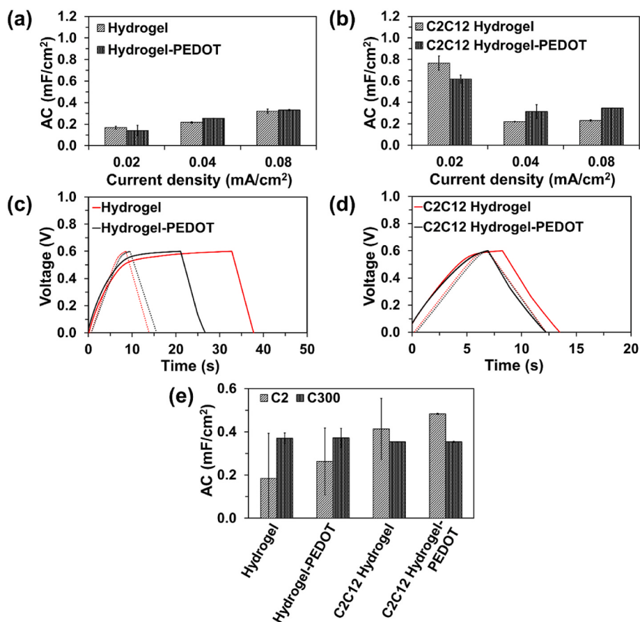
Fig. 8. (a–b) Areal specific capacitance (AC) determined from galvanostatic charge/discharge (GCD) assays at different currents, 0.02, 0.04 or 0.08 \text{mA/cm}^2 ( n = 3 ). (c–d) Cyclability test determined from the 1st and 300th GCD cycle, recorded from 0 to 0.6 V at a current density of 0.04 \text{mA/cm}^2 for (c) Hydrogel, Hydrogel-PEDOT, (d) C2C12 Hydrogel and C2C12 Hydrogel-PEDOT. (e) AC determined from GCD before and after with 300 consecutive GCD cycles ( n = 3 ).
